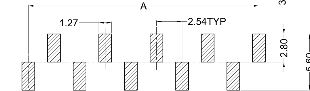
Recommended P.C.B Layout General Tolerance±0.05
